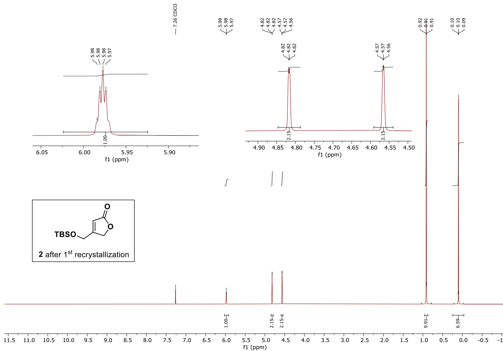
1 H NMR of 2 after 1 recrystallization (500 MHz, CDCl 3 )
